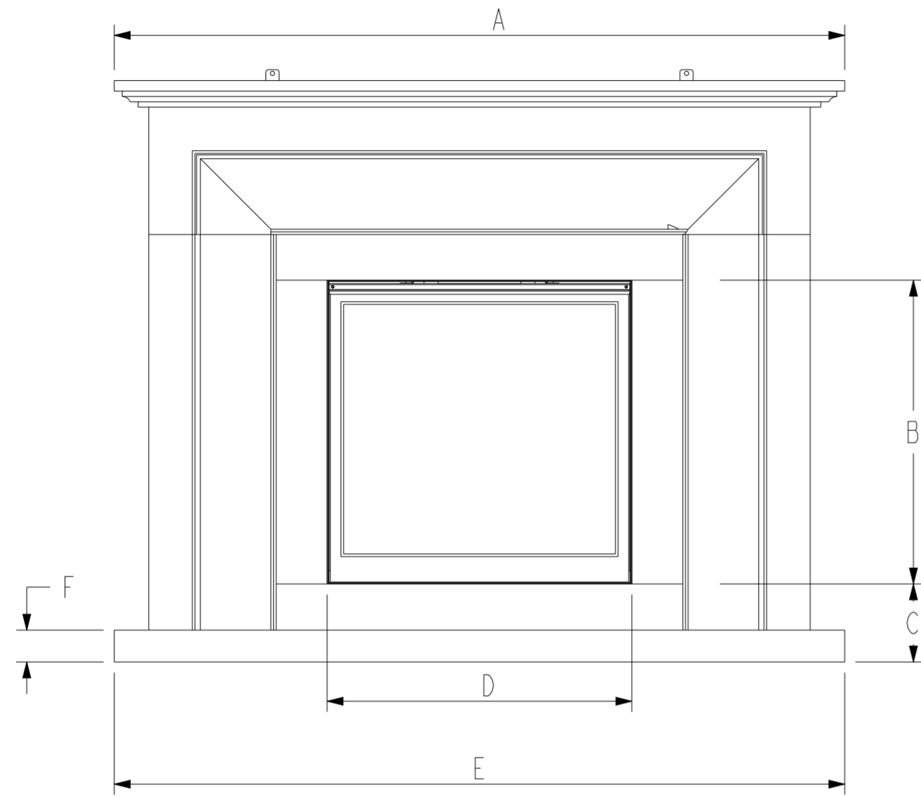
FRONT VIEW
