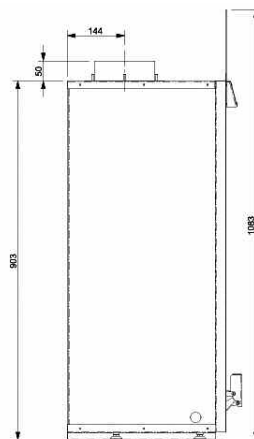
Fig 2 Side View of Combustion Chamber
