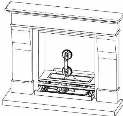
Fig. 14 Drop down the glass assembly to clear top of surround recess
