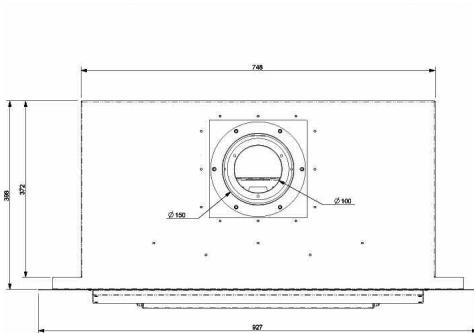
Fig 1 Top View of Combustion Chamber
