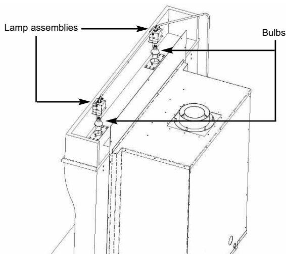
Fig. 30 Shown from rear for clarity
