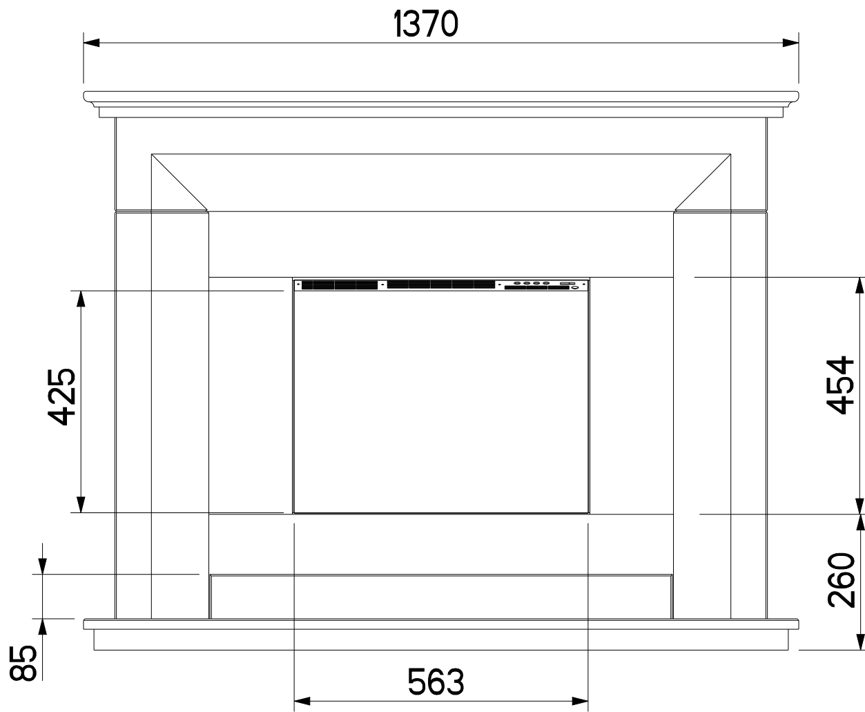
ANGELO ALL DIMENSIONS IN mm
