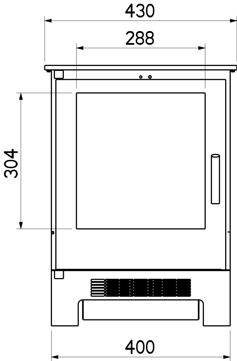
E-VR ARUNDEL STOVE ALL DIMENSIONS IN mm
