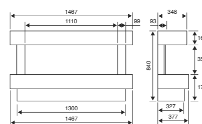
CARINO 1100 ILLUMIA
