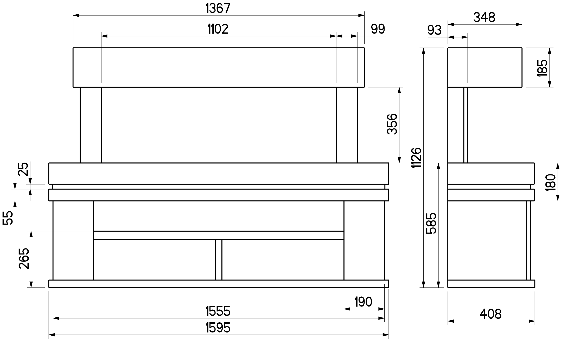
E-VR MEDIA 1100 SUITE ALL DIMENSIONS IN mm
