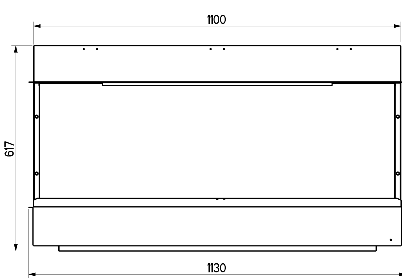
E-VR 1100 ALL DIMENSIONS IN mm
