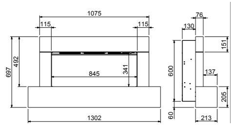
FIREBEAM XL800 ILLUMIA
