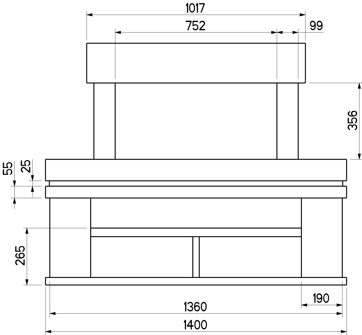
E-VR MEDIA 750 SUITE ALL DIMENSIONS IN mm
