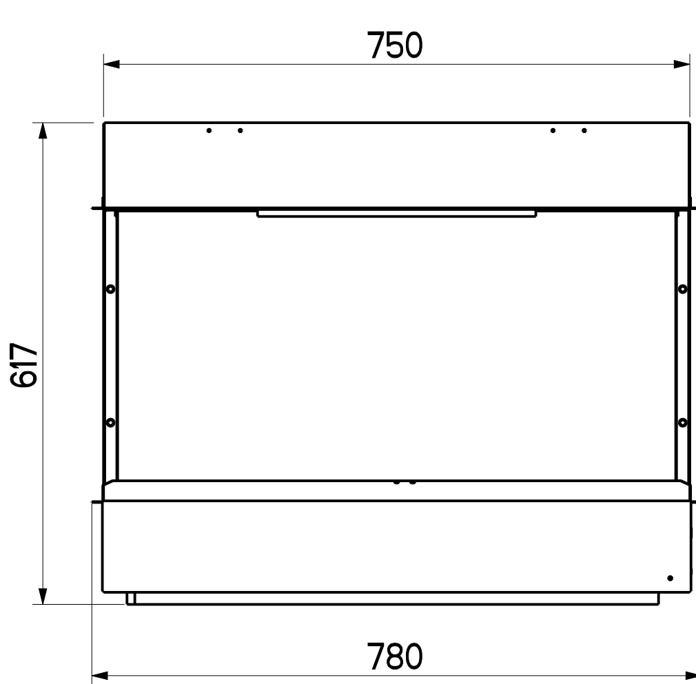
E-VR 750 ALL DIMENSIONS IN mm
