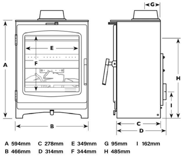
Luxima Wood
