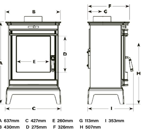
Rochester 5 Wood
