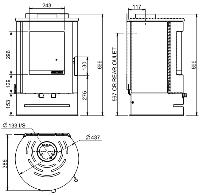
PB 1000 Multifuel
