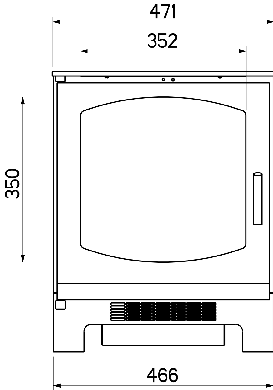
E-VR LUXIMA STOVE ALL DIMENSIONS IN mm
