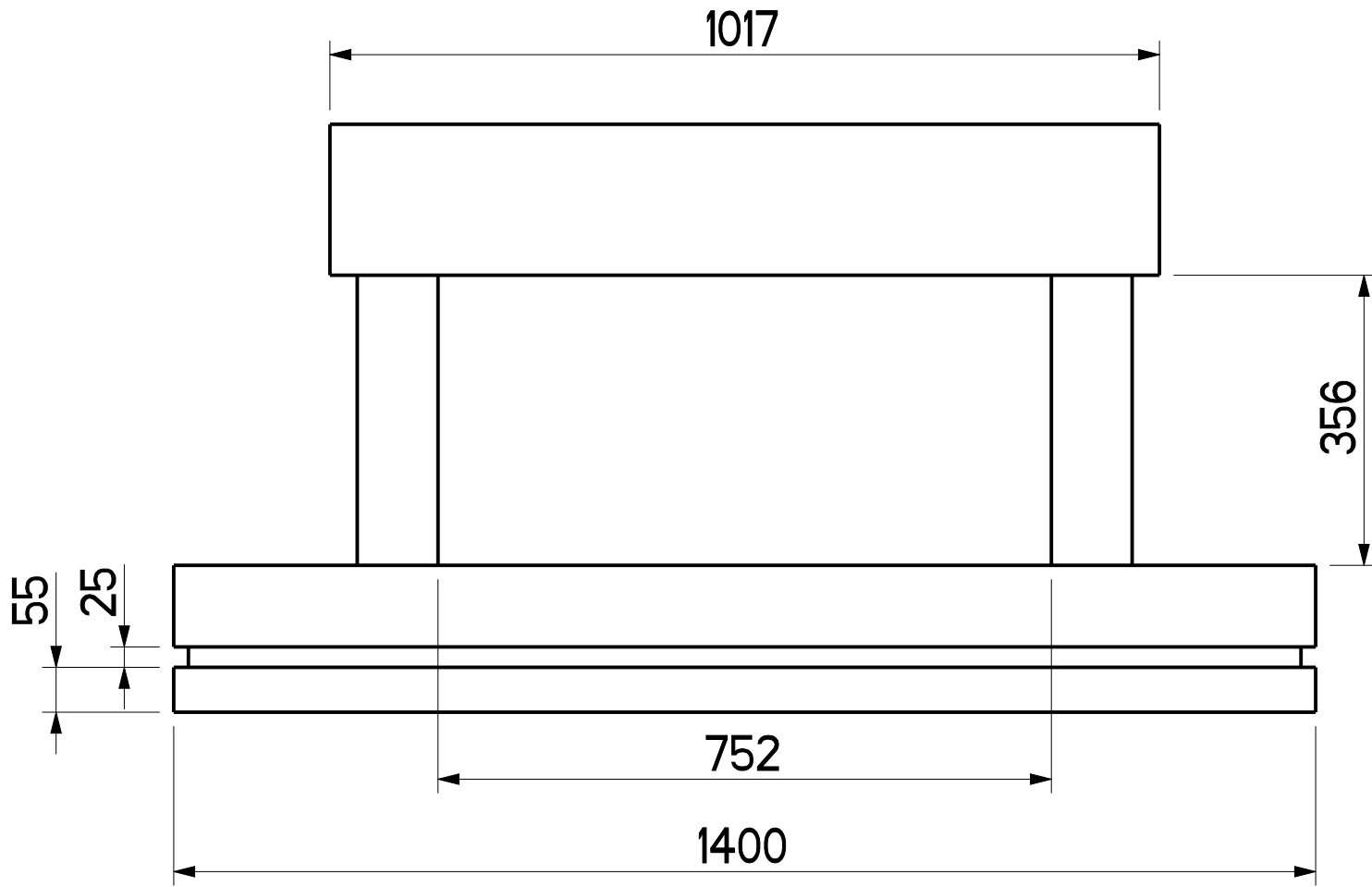
E-VR VOLARE 750 SUITE ALL DIMENSIONS IN mm
